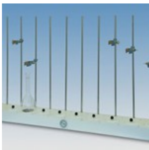
Series Water Baths for EX protection areas
